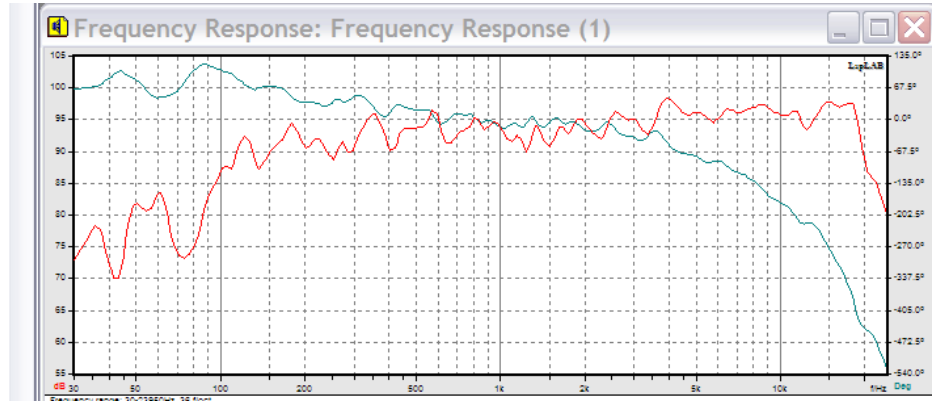
SFR200-A fullrange loudspeaker , AlNiCo TS parameters and frequency response
