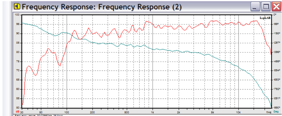
SFR175-A fullrange loudspeaker AlNiCo TS parameters and frequency response
