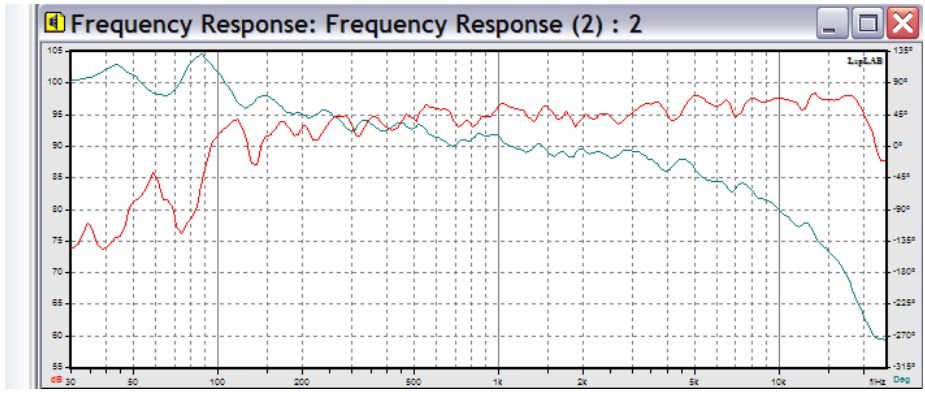
SFR175-8 Fullrange Loudspeaker TS-parameters and frequency response
