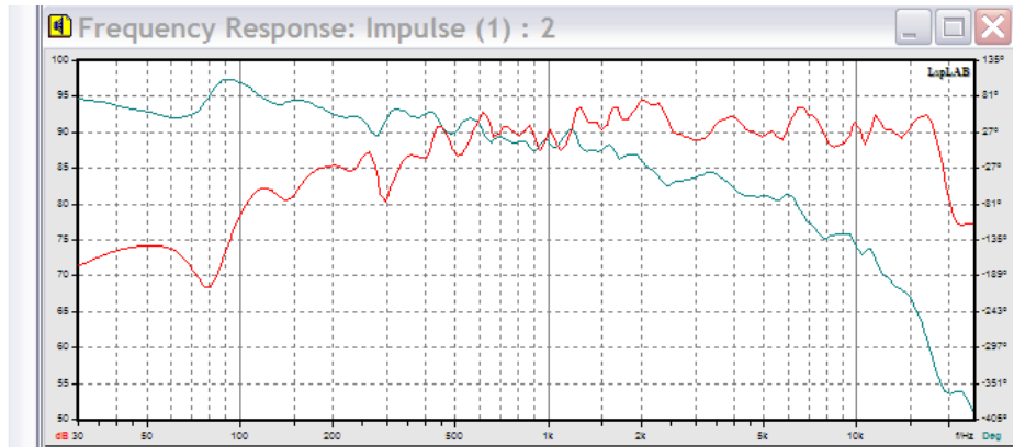
SFR145-8 fullrange loudspeaker, back loaded horn application
