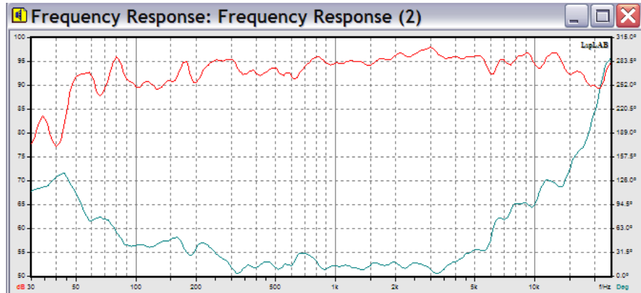
SWR 300 wide range loudspeaker 12" diameter
