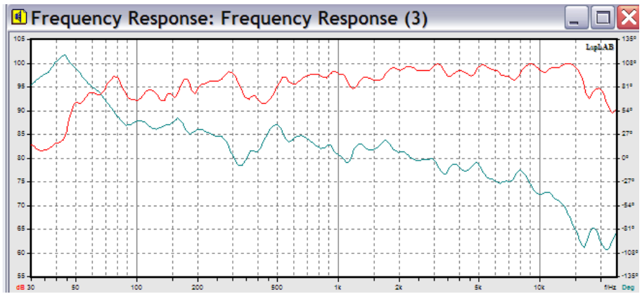
Sonido SWR 250 wide range loudspeaker for bass reflex application
