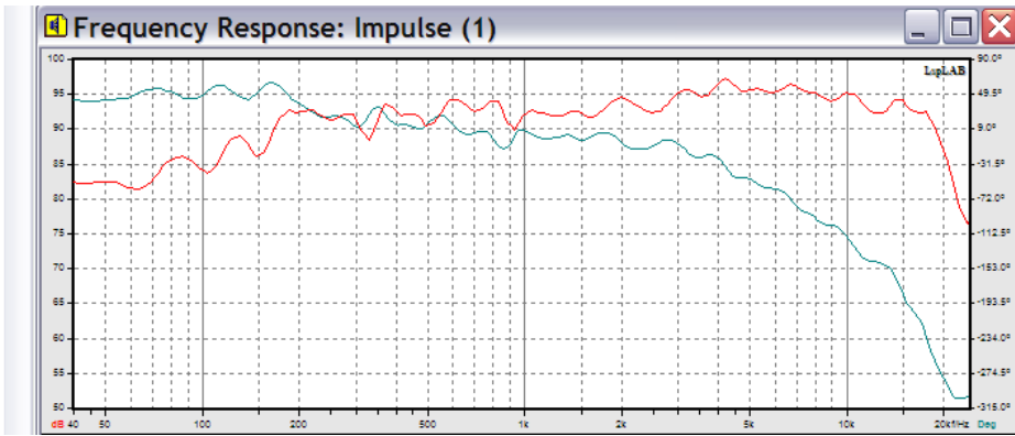
SWR 200-A wide range loudspeaker, AlNiCo, TS parameters and frequency response
