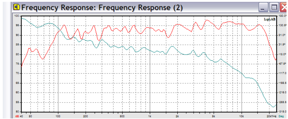
SWR200 wide range loudspeaker TS parameters and frequency response
